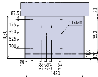
STRATO-Apex 776
